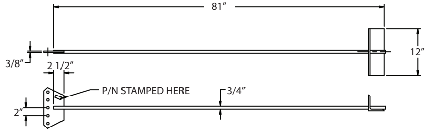
GAC3455STOP ( 17,670 LBS. ALLOWABLE LOAD)*
