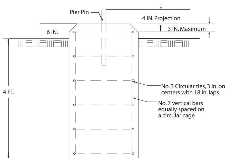
ELEVATION VIEW
