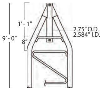
TOP SECTION 45AG5
