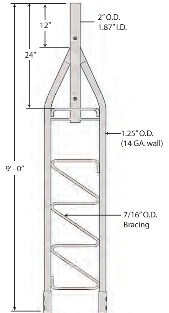
STANDARD TOP SECTION 45AG
