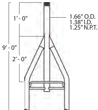
TOP SECTION 45AG1
