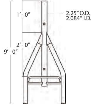
TOP SECTION 45AG3
