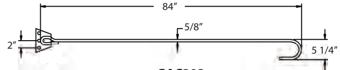
GAC303 ( 7,330 LBS. ALLOWABLE LOAD)*
