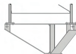
STANDARD TAPERED BASE 45GSRTB
